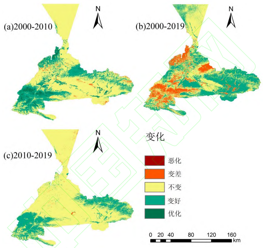
图 4 2000—2019 年乌鲁木齐市 RSEI 变化监测 Fig.4 Change detection diagram of RSEI in Urumqi City from 2000 to 2019
