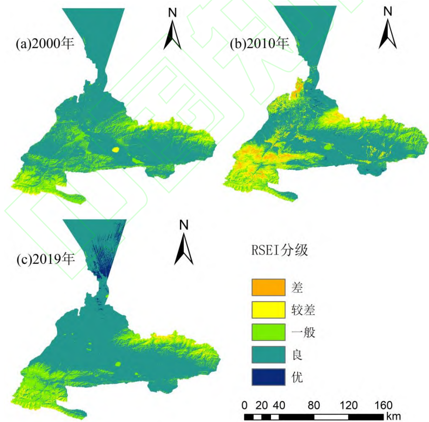
图 2 乌鲁木齐市遥感生态指数的等级分布 Fig.2 Spatial distribution remote sensing ecological index value classes in Urumqi City
