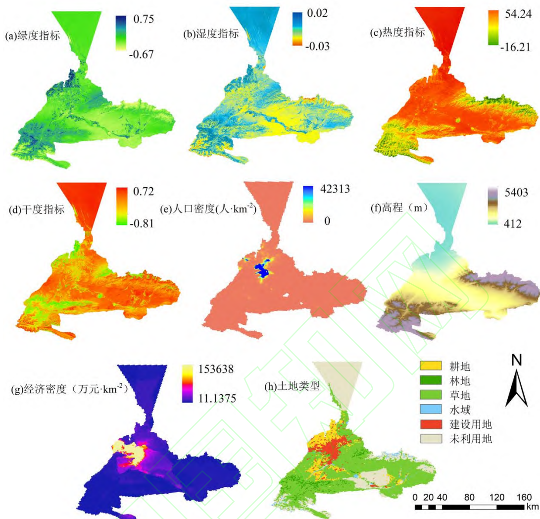
图 5 探测因子空间分布 Fig.5 Risk detection and interactive detection matrix
