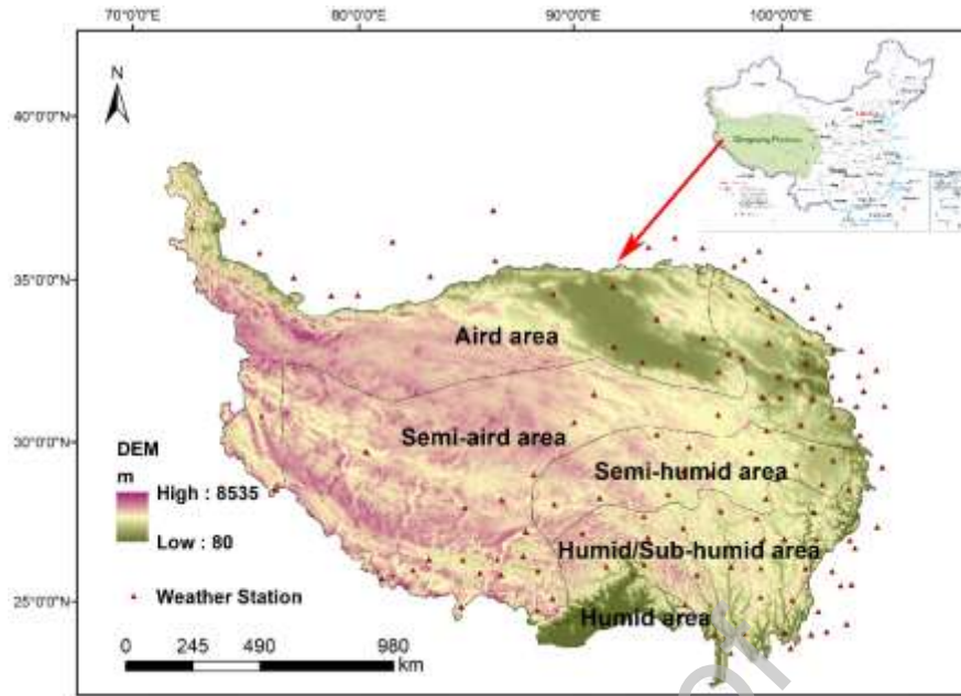
Fig. 1. The eco-geographical regions of the Qingzang Plateau, in China.
