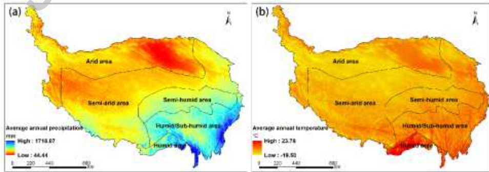
Fig. 2. Annual average (a) precipitation and (b) temperature.
