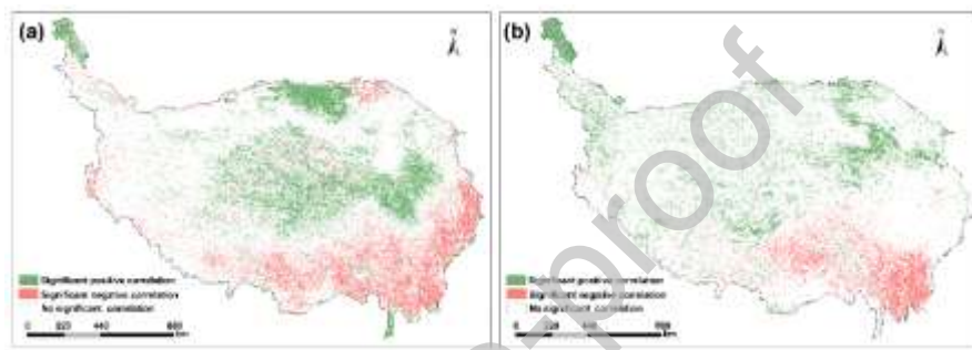
Fig. 8 Spatial variation in correlations between average annual NDVI and temperature (a) and precipitation (b). Notes: Correlation is significant at the 0.05 level (2-tailed).
