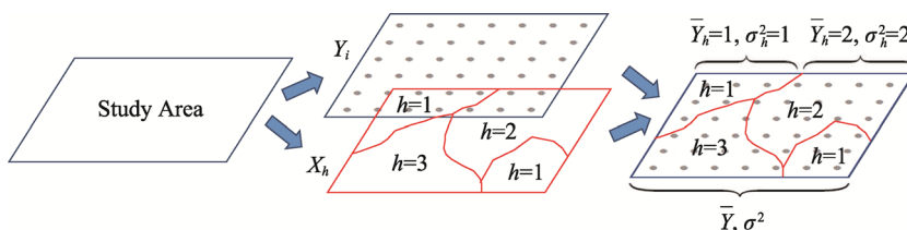
Figure 5 Principle of the geographical detector (after Wang and Xu, 2017)
