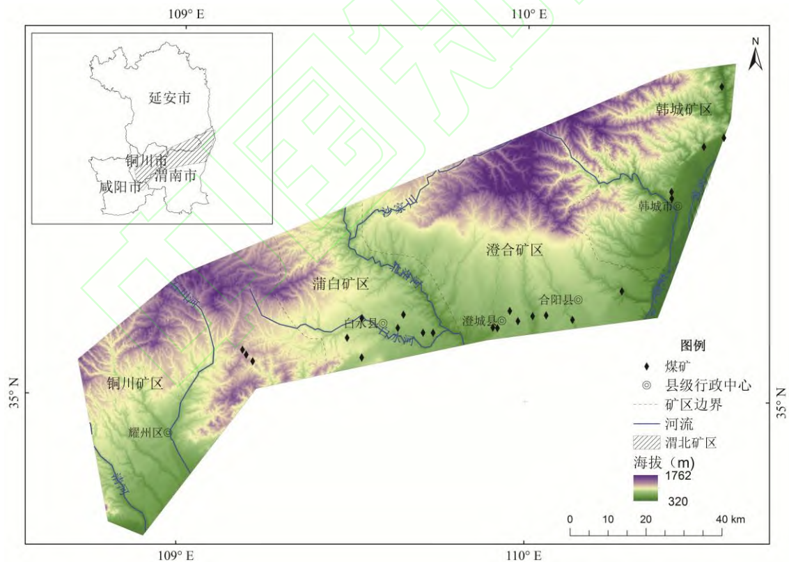
图 1 渭北矿区地理位置示意图实验 Fig. 1 Geographical location of the Weibei mining area
