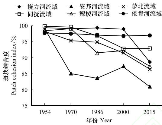
图 4 1954—2015 年三江平原子流域沼泽湿地斑块结合度变化图 Fig.4 The variation of patch cohesion index of swamps in sub-basins of the Sanjiang Plain from 1954 to 2015
