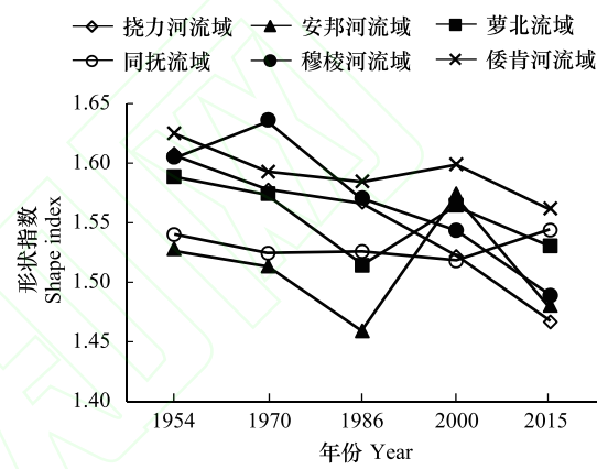
图 5 1954—2015 年三江平原子流域沼泽湿地形状指数变化图 Fig.5 The variation of shape index of swamps in sub-basins of the Sanjiang Plain from 1954 to 2015
