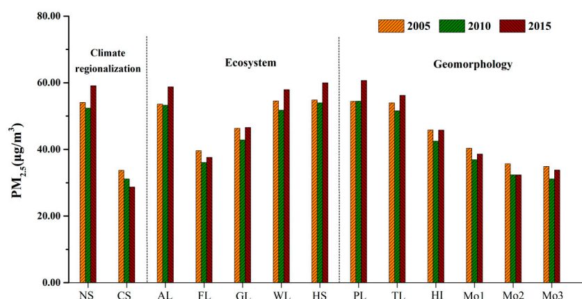
Figure 7. Annual average PM_{2.5} concentrations in different climate, ecosystem and geomorphological subregions (NS = North subtropical humid zone, CS = Central subtropical humid zone, AL = Arable land ecosystem, FL = Forest ecosystem, GL = Grassland ecosystem, WL = Water and wetland ecosystem, HS = Human settlement ecosystem, PL = Plain, TL = Tableland, HI = Hills, Mo1 = Small-undulating mountain, Mo2 = Mid-undulating mountain, Mo3 = Large-undulating mountain).
