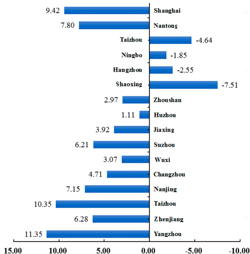
Figure 5. Average annual changes in PM 2.5 concentrations ( \mu\text{g}/\text{m}^3 ) in different YRD cities from 2005 to 2015.
