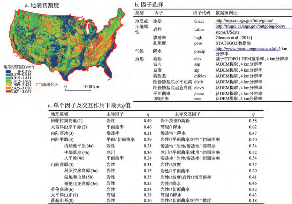
Fig. 8 Risk area detector (a), Risk factor detector (b), Ecological detector (c) and Interaction detector (d)
